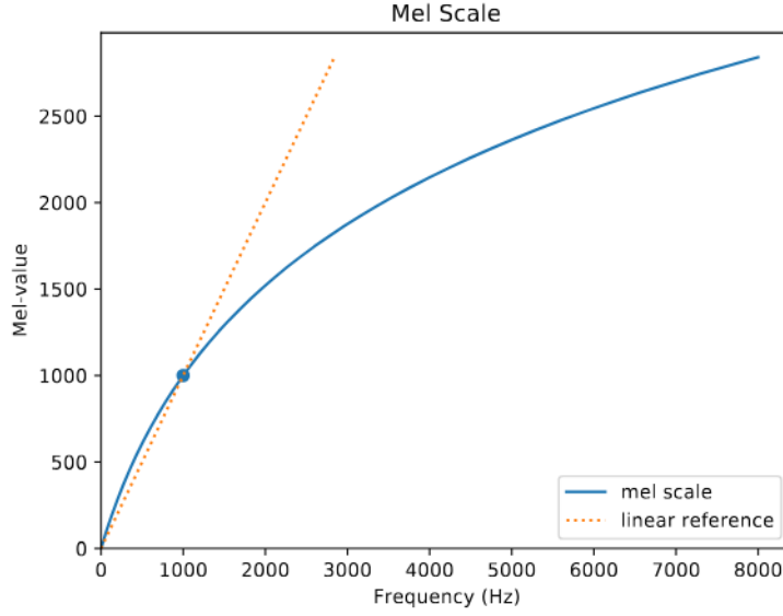
Figure 2.3: Mel values compared to their corresponding frequencies. The dot illustrates the break point at which the perception of pitch difference is lower than the actual change in frequency.
