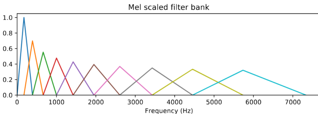
Figure 2.4: A Mel-scaled set of filters with a linear spacing of 250 Mel. Each color represents one filter.
