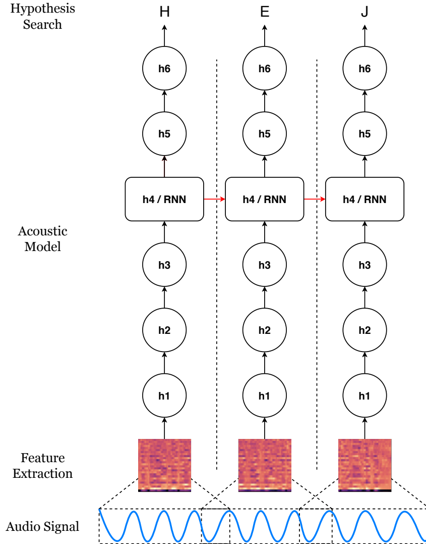
Figure 2.7: Simplified architecture of Mozilla's DeepSpeech model. Each circle represents a layer of several nodes.
