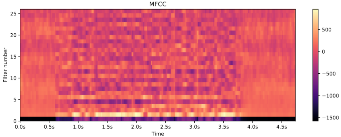
Figure 2.5: MFCC representation of a short audio file from the NST Dataset.
