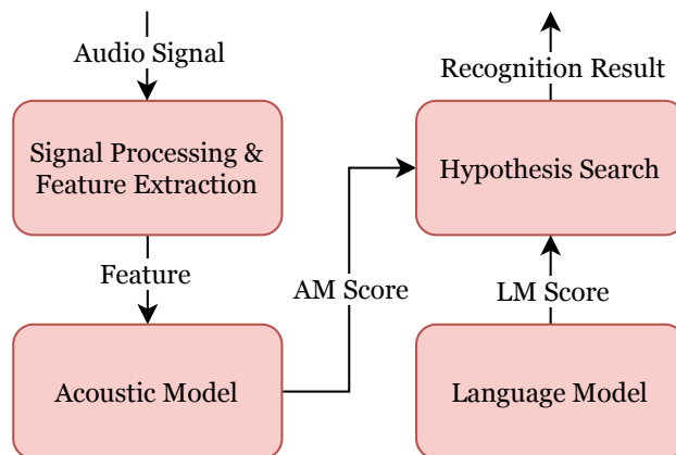
Figure 2.6: Architecture of a typical automatic speech recognition system.
